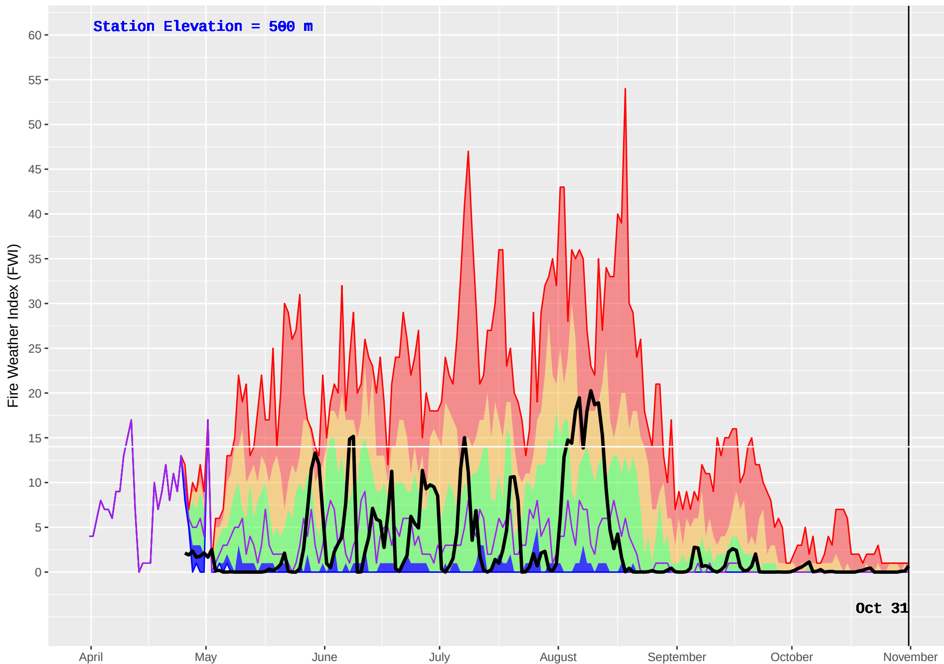
CRANBERRY (433) : Historical (1995–2016) and Current (2017) Noon Fire Weather Index (FWI)
