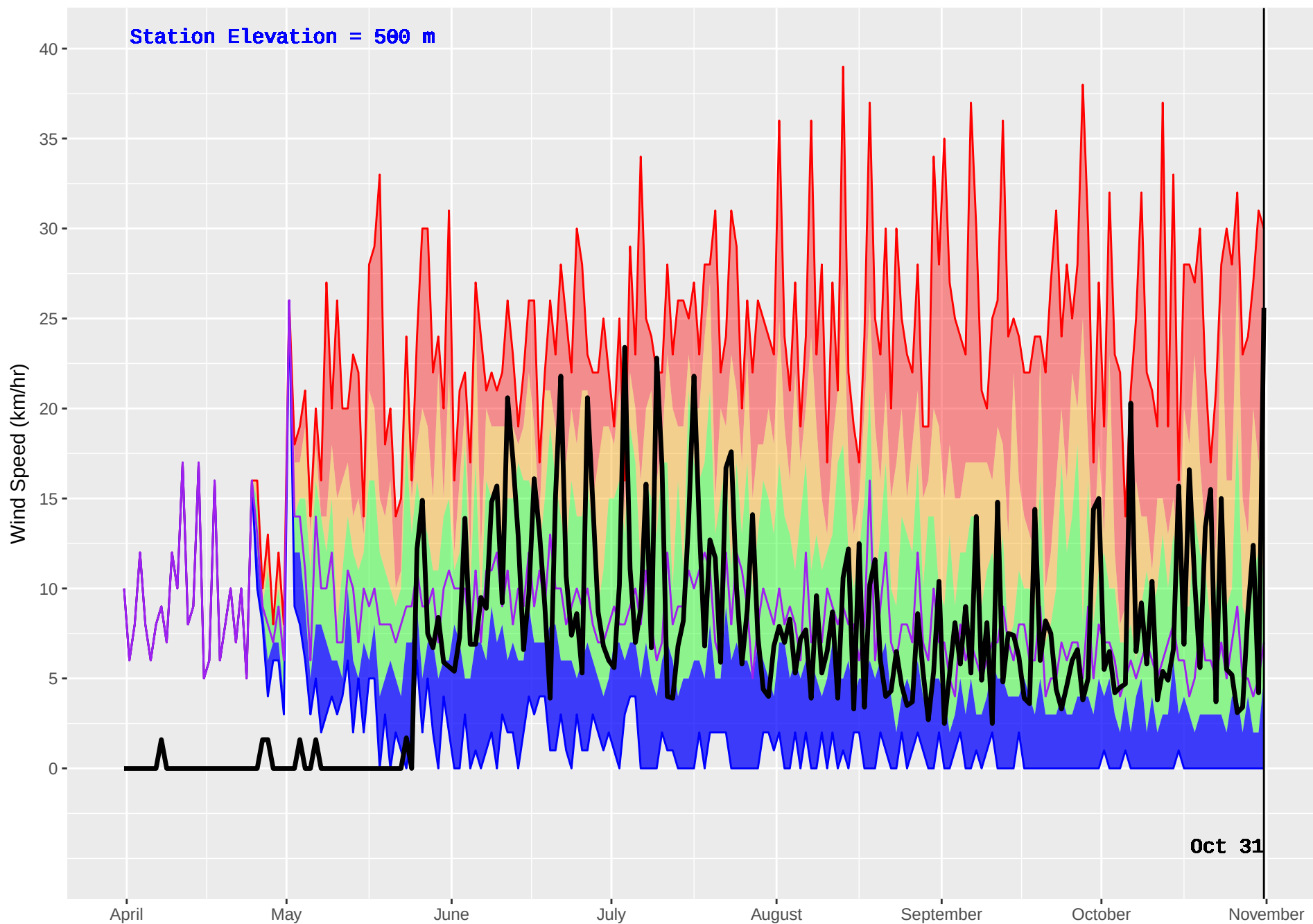
CRANBERRY (433) : Historical (1995–2016) and Current (2017) Noon Wind Speed
