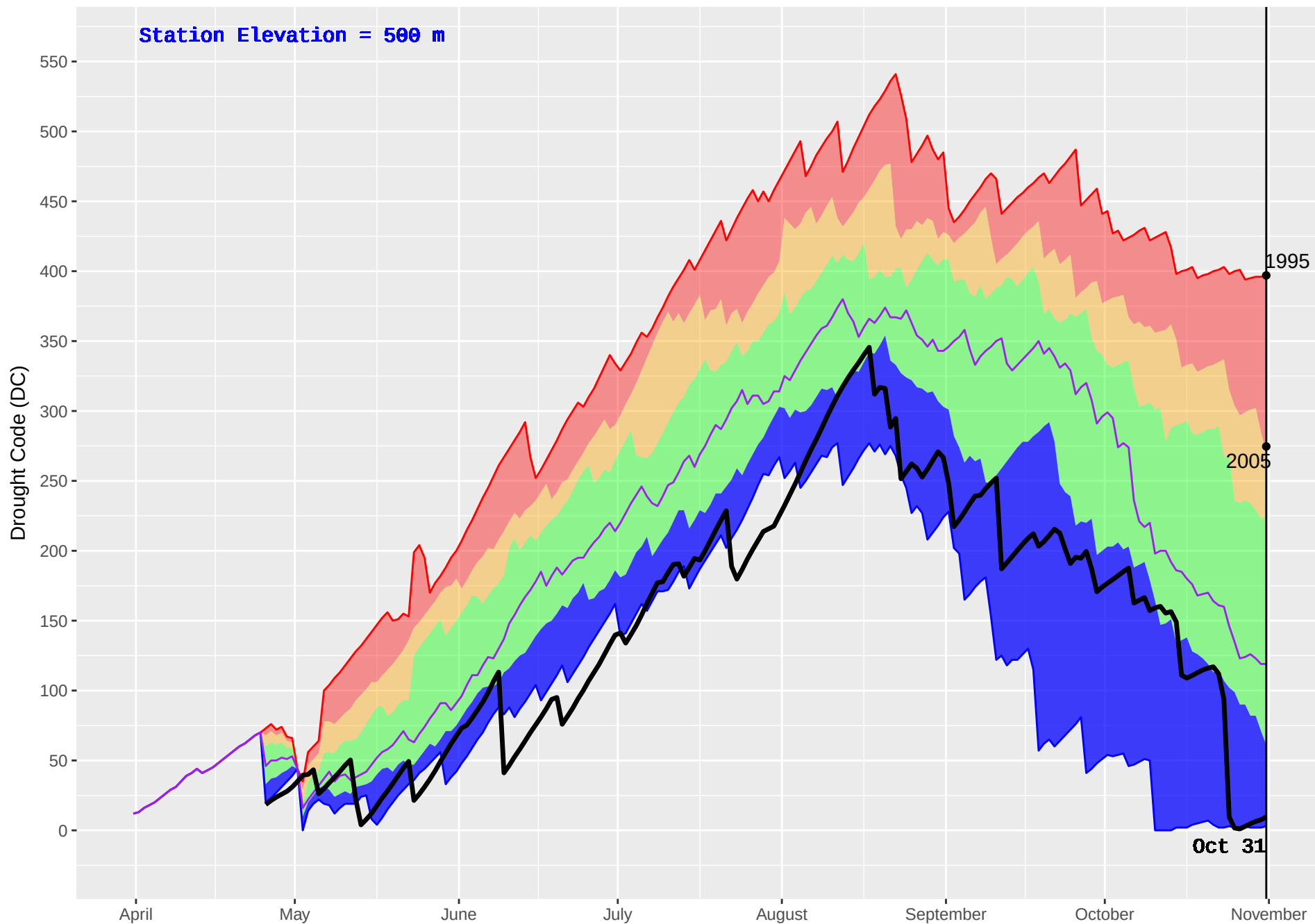
CRANBERRY (433) : Historical (1995–2016) and Current (2017) Noon Drought Code (DC)
