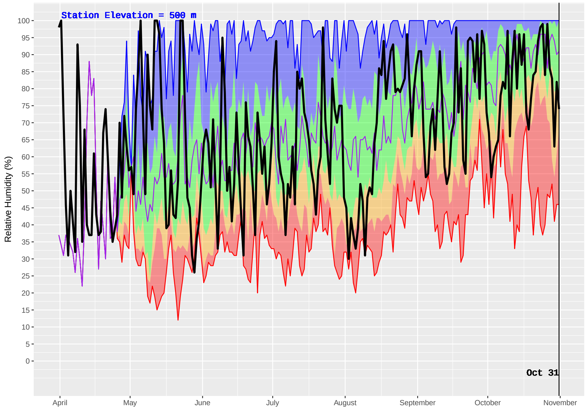
CRANBERRY (433) : Historical (1995–2016) and Current (2017) Noon Relative Humidity
