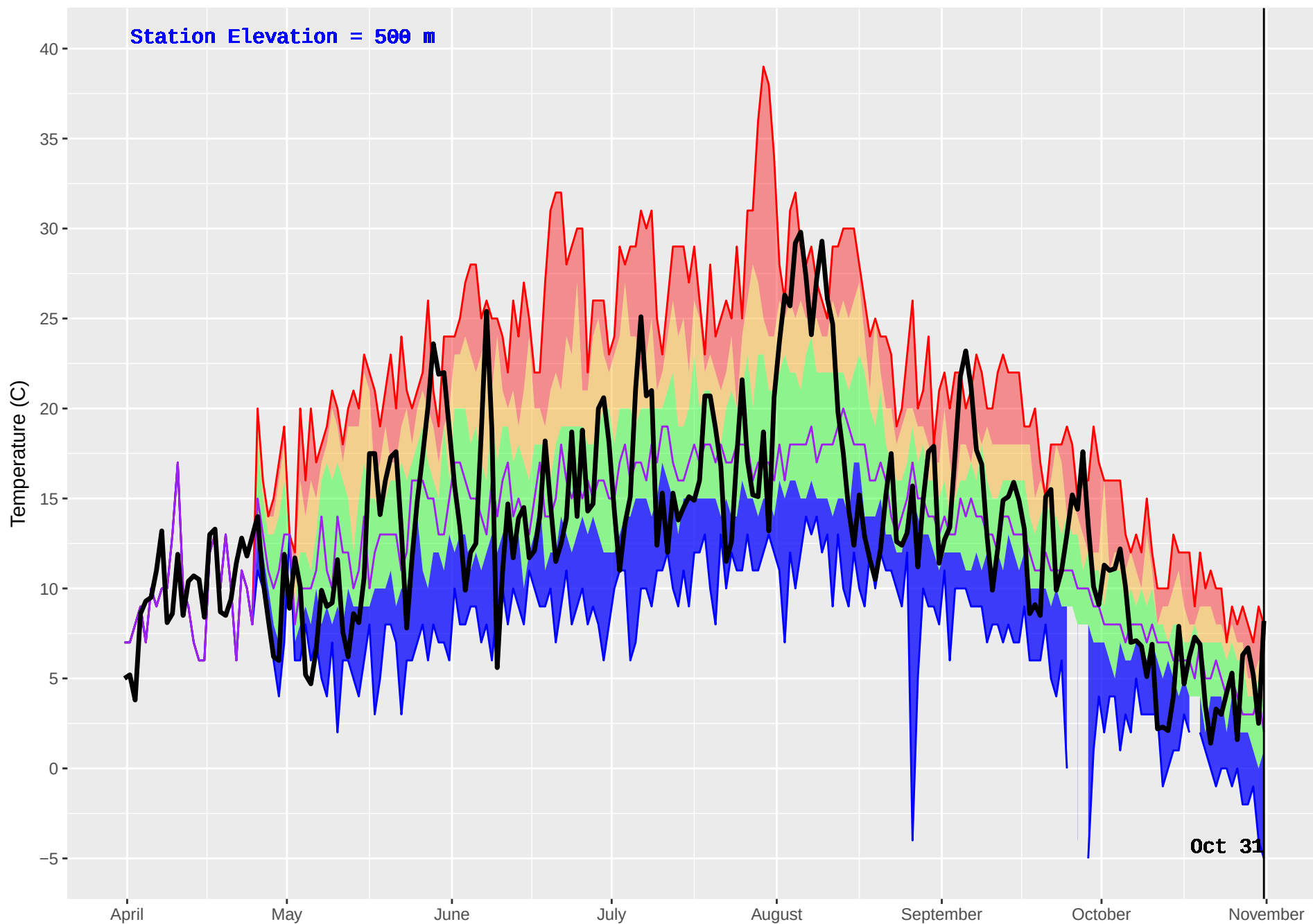
CRANBERRY (433) : Historical (1995–2016) and Current (2017) Noon Temperature
