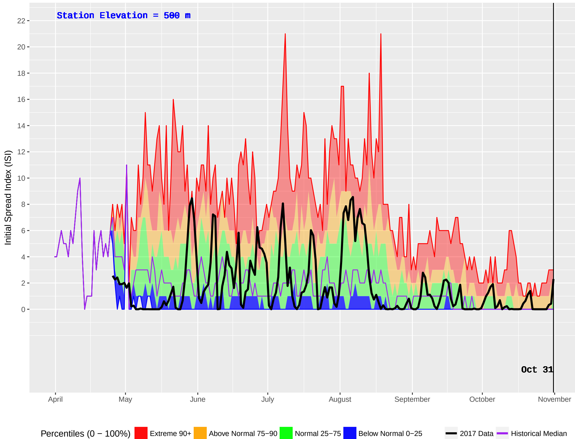
CRANBERRY (433) : Historical (1995–2016) and Current (2017) Noon Initial Spread Index (ISI)
