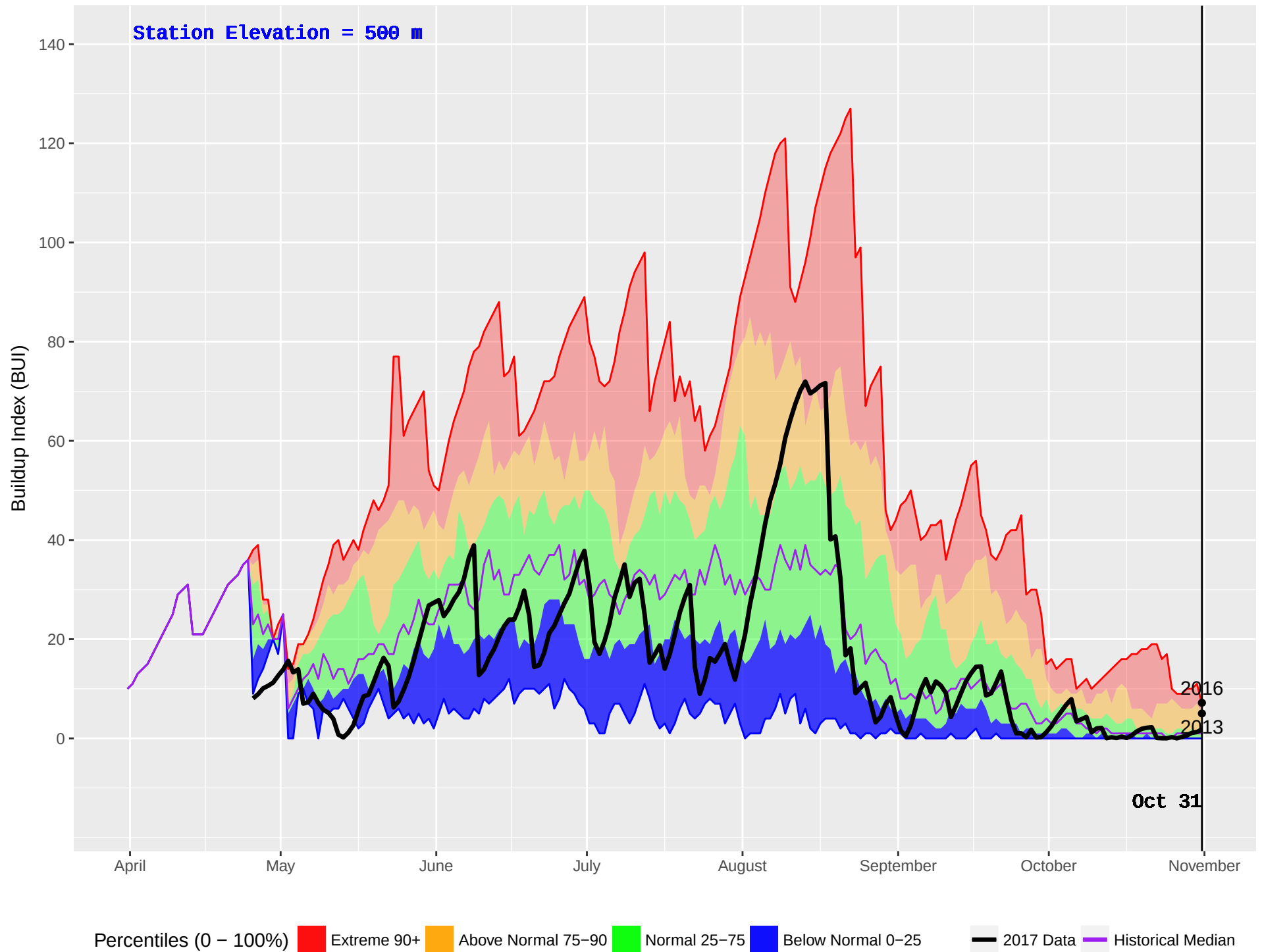
CRANBERRY (433) : Historical (1995–2016) and Current (2017) Noon Buildup Index (BUI)
